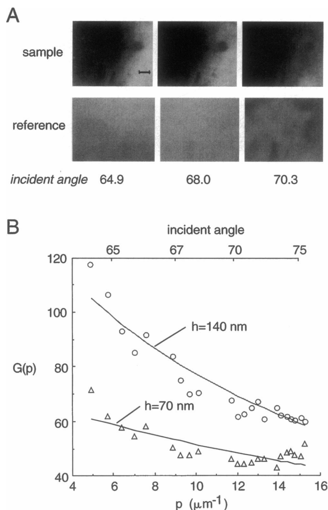
FIGURE 5 Evaluation of MA-TIRFM instrument performance using a curved film of fluorescent solution. The solution film was created as shown in Fig. 2 and described in the text. (A) Fluorescence intensity images of the sample (silica lens in contact with prism, top) and reference (silica lens raised above prism, bottom). Representative images shown for 3 of 22 incident angles. Bar, 5 \mu\text{m} . (B) Nonlinear regression of angle-resolved intensity distributions shown for two randomly chosen pixels (of 64,000 pixels). Data were fitted to a top-hat function (Eq. 6) with fitted h values as shown.
