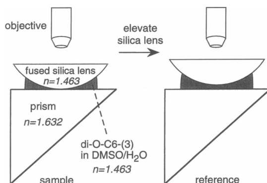
FIGURE 2 Evaluation of MA-TIRFM instrument performance using a known fluorophore distribution. A spherical film of di-O-C6-(3) in DMSO/water was created by making point contact between a fused silica plano-convex lens and the F2 glass prism ( left ). A uniform "reference" fluorophore distribution was created by raising the silica lens by \sim 1 \mu m ( right ).
