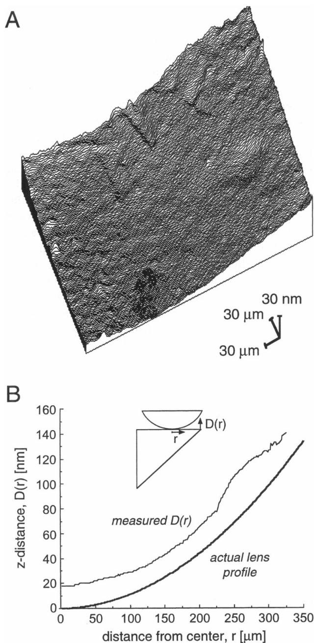
FIGURE 6 3-d distribution of solution thickness from data set shown in Fig. 4. (A) 3-d contour plot reconstruction of the fluid layer between the flat prism ( bottom ) and curved surface of plano-convex lens ( top ). (B) Solution thickness as a function of distance from lens-prism contact point, D(r) , determined by radial averaging of data from (A). Actual lens profile determined from manufacturers specification of 458 nm lens radius.
